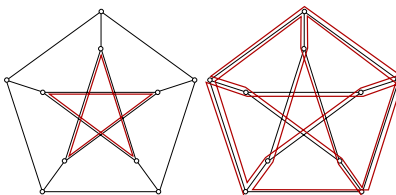
FIGURE 17. The two geodesics of the Petersen graph.
